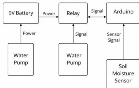
Fig. 1. System block diagram of the Smart Irrigation System.
