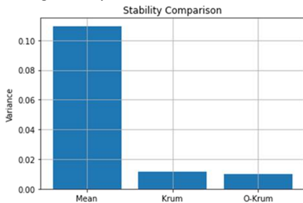
Fig. 4 Variance Comparison
