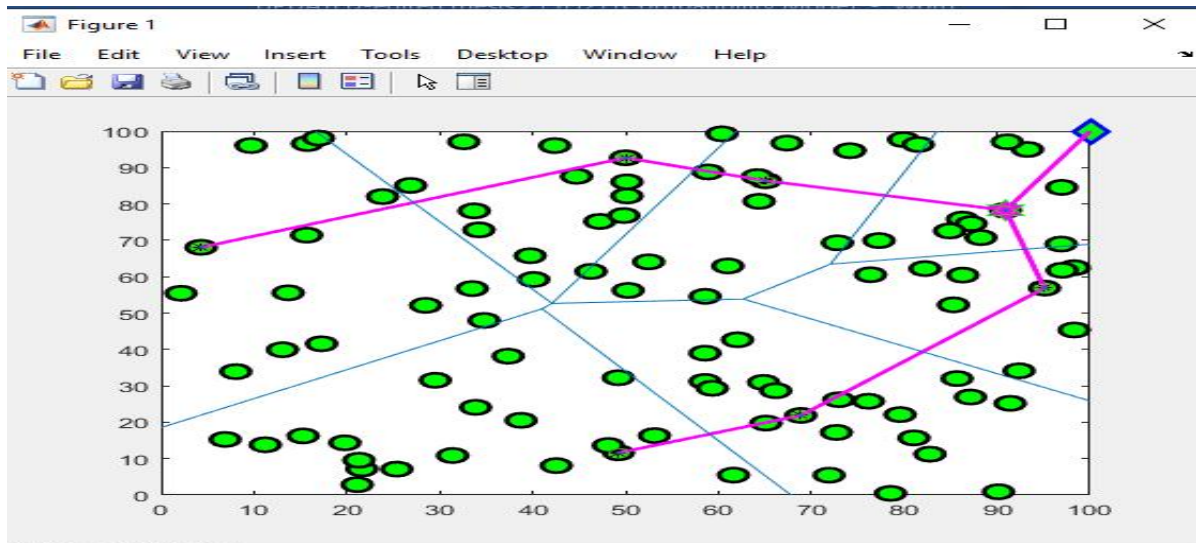
Figure 4.4 : Nodes Structure
