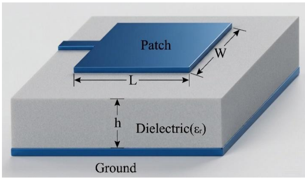
Fig. 1 Structure of Microstrip Patch Antenna [5]
