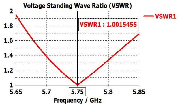
Fig. 4 VSWR of the Antenna
