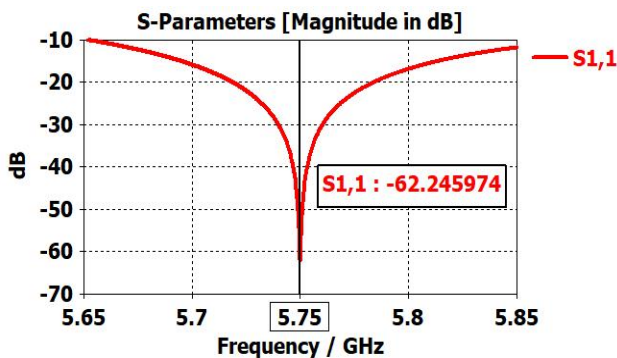
Fig. 3 Return Loss of the Antenna
