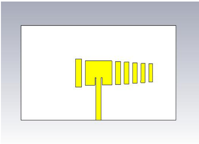
Fig. 2 Two-dimensional model of designed microstrip patch Yagi-Uda antenna
