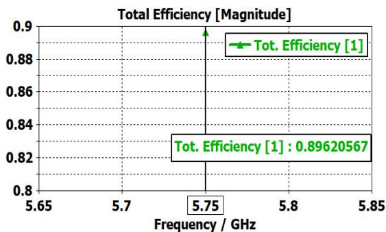
Fig. 7 Efficiency graph of the Antenna
